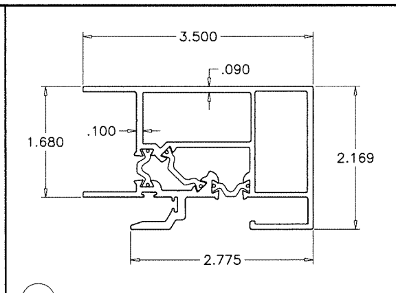
E6 STD. INTERIOR INTERLOCK
