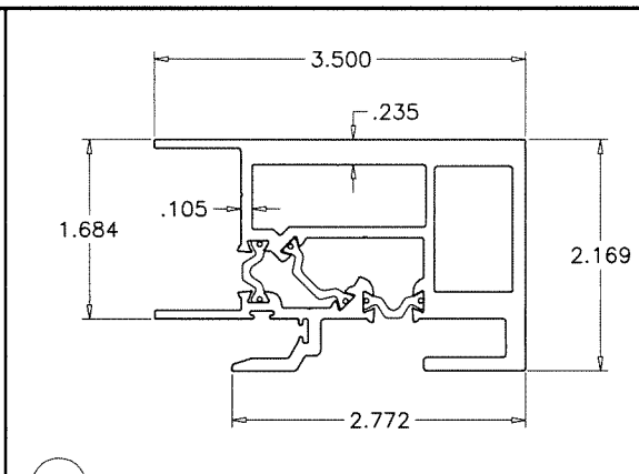
E6B H.D. INTERIOR INTERLOCK
